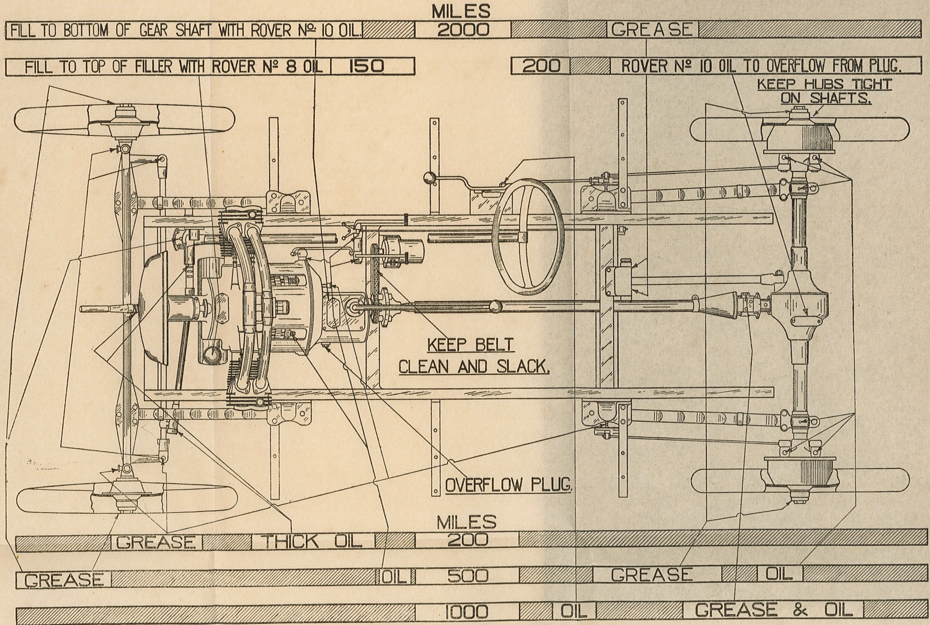
INSTRUCTION AND OILING DIAGRAM. 8 H.P. ROVER CAR.
